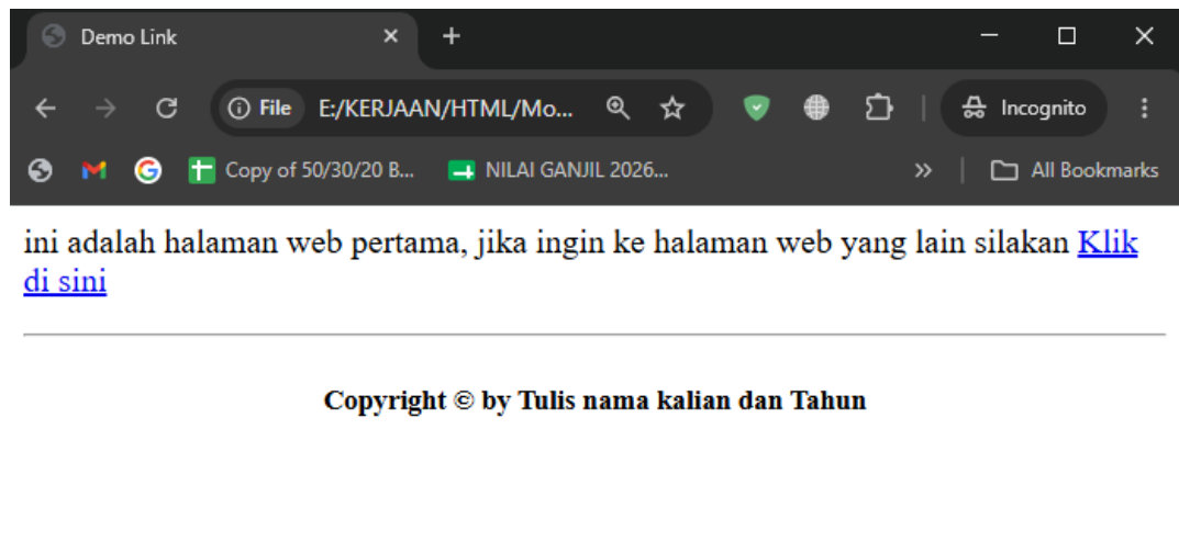
Gambar 1.1 Tampilan program 1.1
