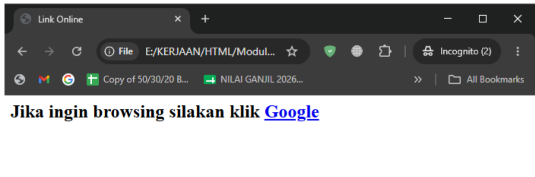
Gambar 1.6 Tampilan program
